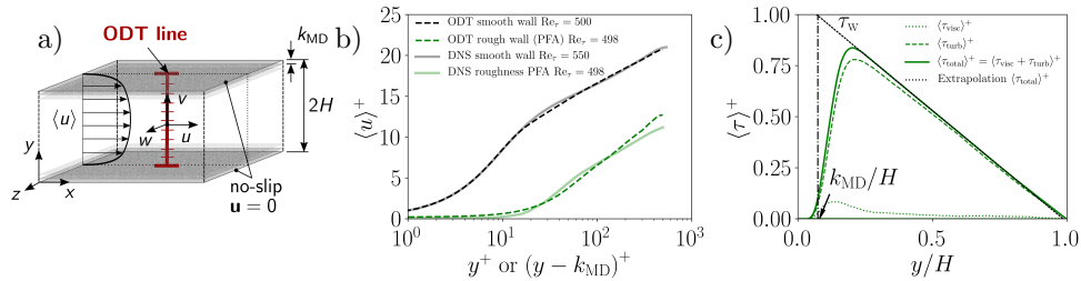
Figure 1: (a) Sketch of the configuration. (b) Mean velocity \langle u \rangle boundary layer for ODT and DNS 3,7 (melt-down height k_{MD}^+ = 67 , k_{MD}/H = 0.12 ) demonstrating absence of the buffer layer over roughness. (c) ODT turbulent and total stress \langle \tau \rangle with indication of the equivalent smooth-wall location obtained by extrapolation with the wall-shear stress \tau_w . The superscript (\cdot)^+ denotes inner scaling.
