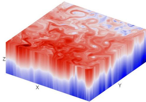
Figure 1: Visualisation of mesoscale eddies in a simulation of an idealized patch of ocean using the total temperature field.
